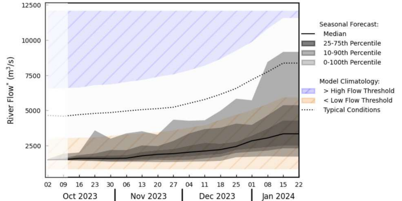
Hydrograph
