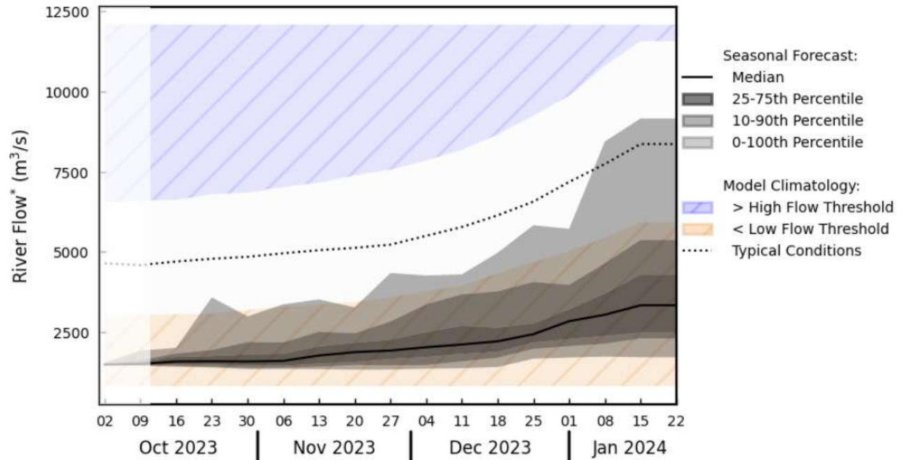
Hydrograph
